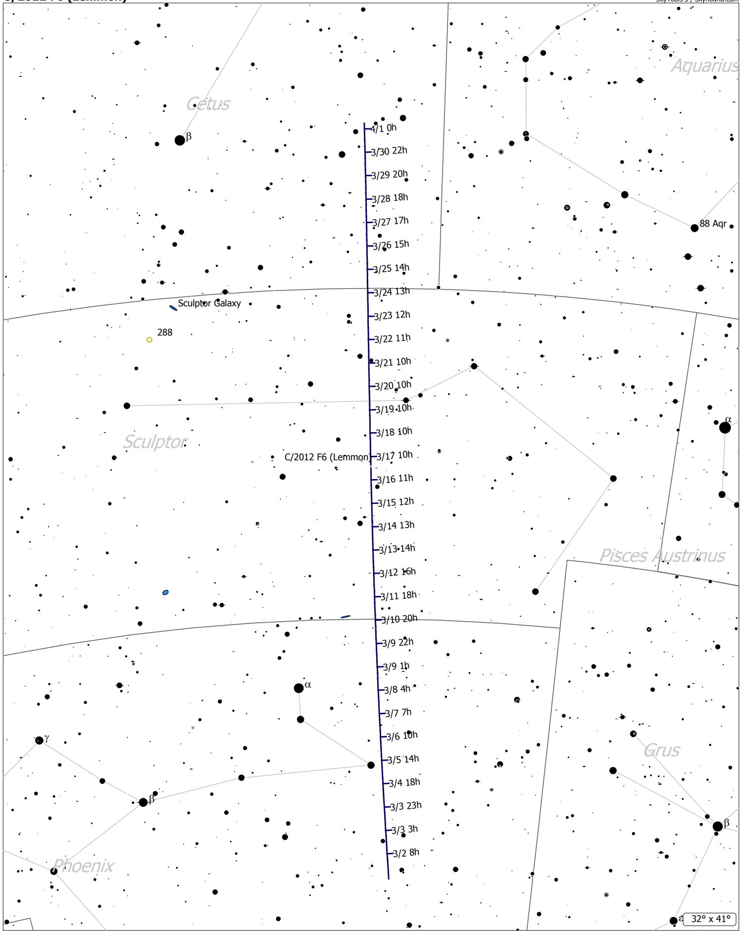
C/2012 F6 (Lemmon) (Comet) Magnitude: 4.92 Coma Diameter: 23" SBr: 11.5 Mag/arcsec 2 Earth
